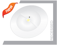
Model : PEL 1W LED NM/RDL (CR) Lamp Type : 1 Watt LED Accumulator : Ni-Mh / Ni-Cd Battery Backup : 3 Hrs. Standard Pkg.: 10 pcs. Box size in mm : 355x215x415
