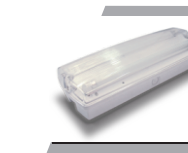
Model : PEL LED M/WP (1) Lamp Type : 1 x 8W T5 FTL Accumulator : Ni-Cd Battery Backup : 2 Hrs. Standard Pkg.: 10 pcs. Box size mm : 490x305x400
